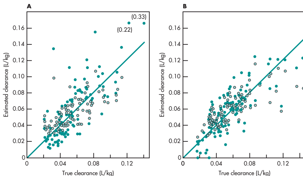
FIGURE 22-4 Plots of predicted clearance versus true (simulated) clearance for predictions by the Bayesian (<inline>) and alternative (<inline>) methods. The diagonal line on each graph is the line of identity. A shows results for one-sample group; B shows results for two-sample group. (From Sheiner and Beal, 1982, with permission.)
