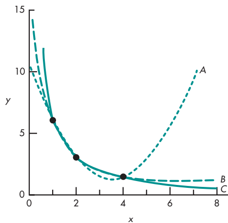
FIGURE 2-6 Three points equally well fitted by different curves. The parabola, y = 10.5 - 5.25x + 0.75x^2 (curve A); the exponential, y = 12.93e^{-1.005x} + 1.27 (curve B); and the rectangular hyperbola, y = 6/x (curve C) all fit the three points (1,6), (2,3), and (4,1.5) perfectly, as would an infinite number of other curves. (Reprinted with permission from Riggs DS: The Mathematical Approach to Physiological Problems . Baltimore, Williams & Wilkins, 1963.)
